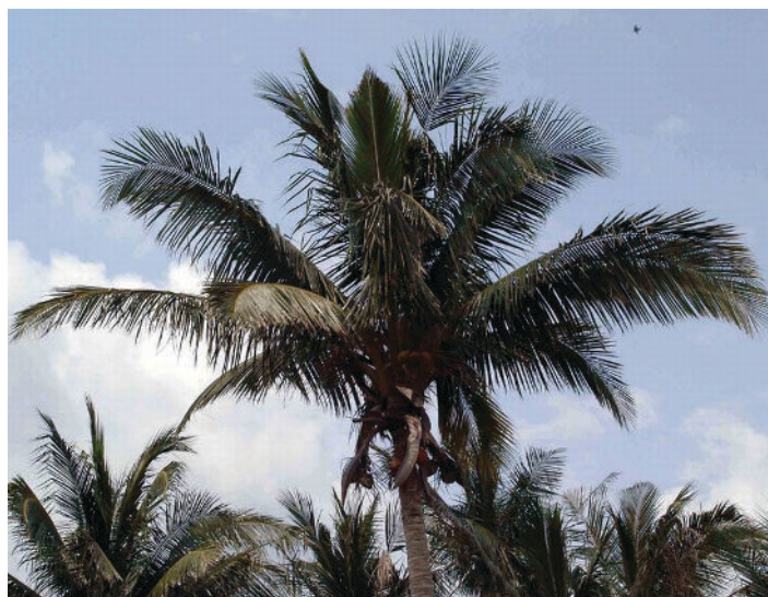
Figure 20. A typical coconut palm ( Cocos nucifera ) in South Florida holding only 13 leaves due to K deficiency.
